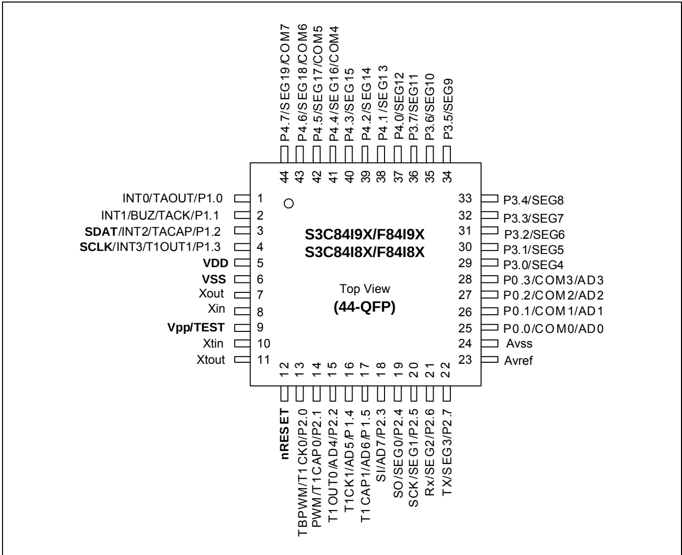
图 1-2 S3C84I8X/F84I8X/C84I9X/F84I9X管脚分布图 (44- QFP)
